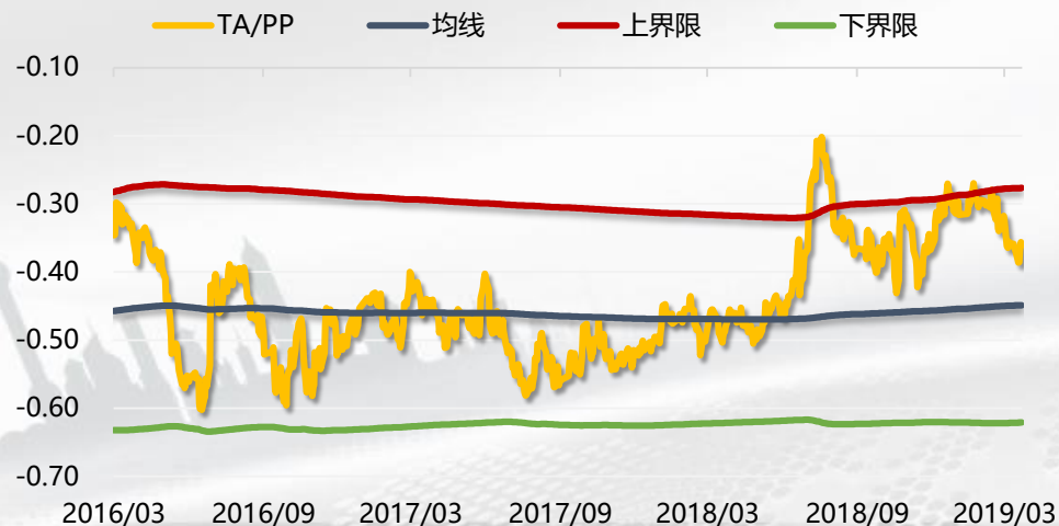
TA/PP价比观测
